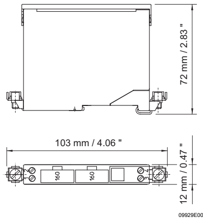
Safety barriers 9001, 9002, 9004
