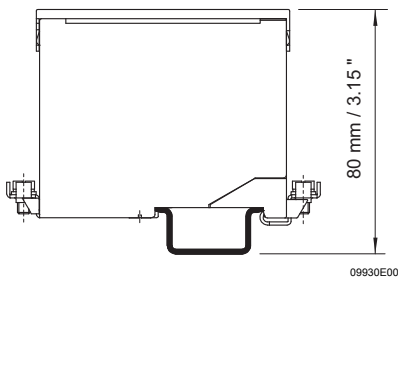
Safety barrier 9001, 9002, 9004 mounted on the mounting rail LV 35/15
