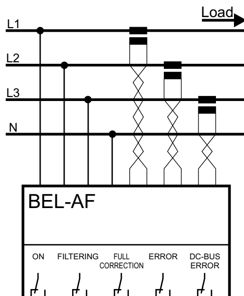
open loop
