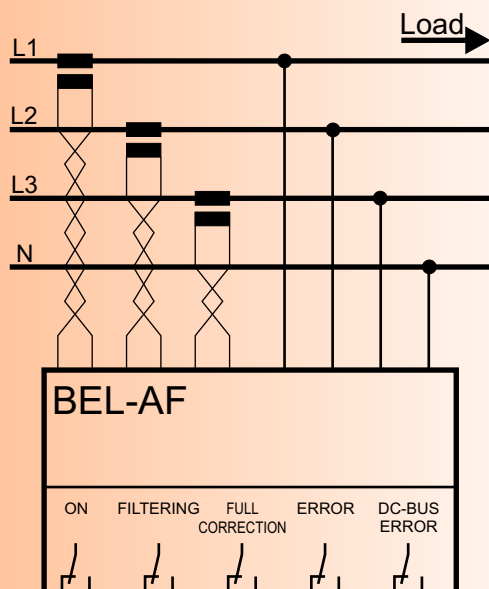
closed loop
