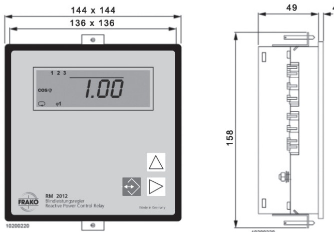
Dimensional drawing RM 22012 6+6D/12D
